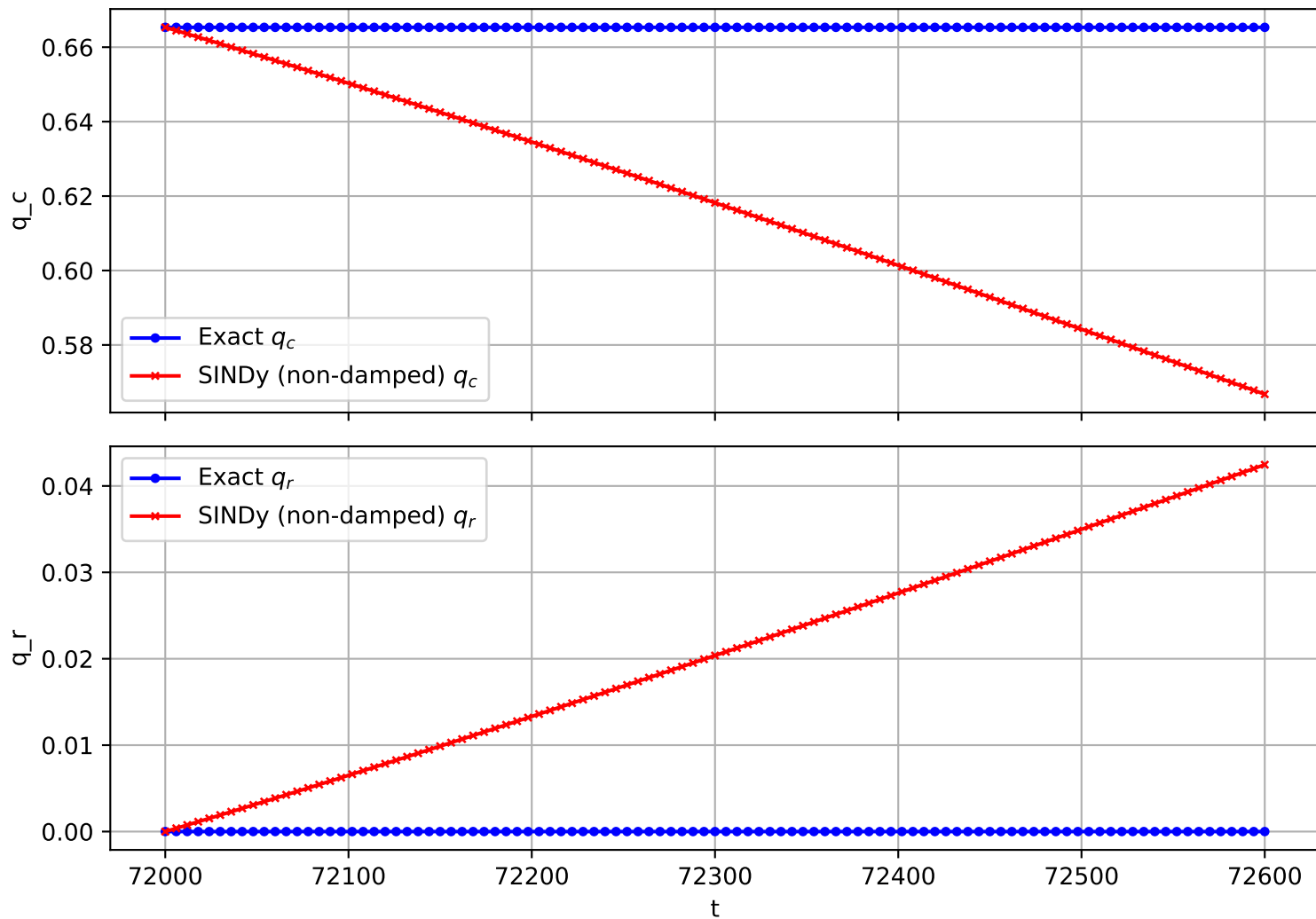
Trajectory 162 (non-damped)
