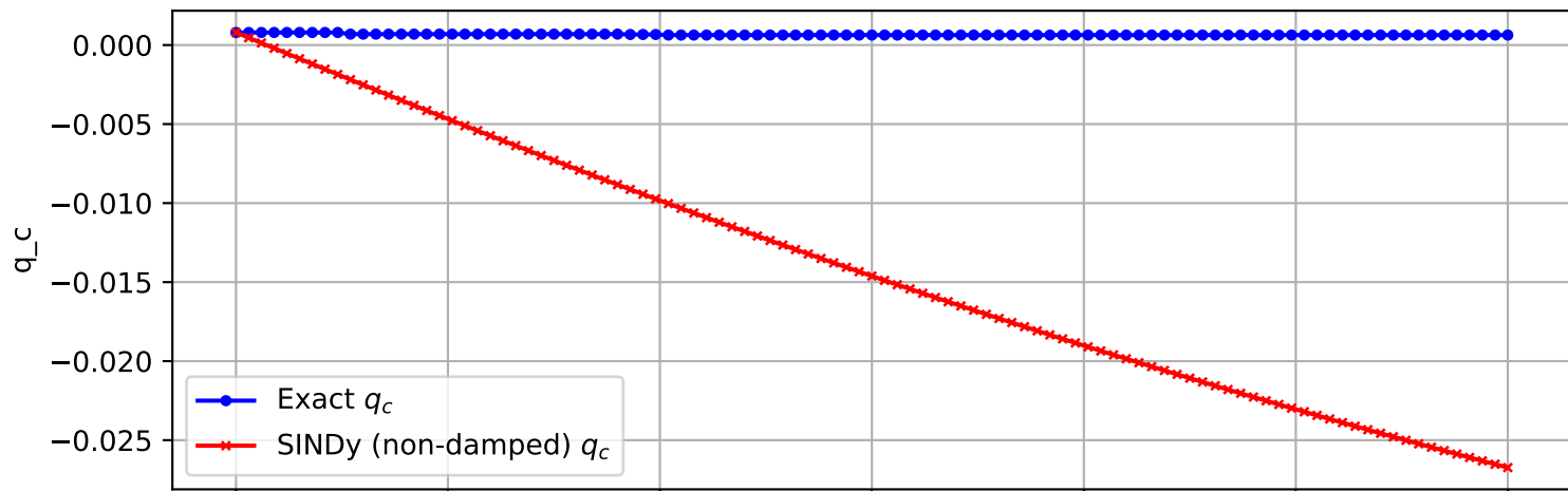
Trajectory 1623 (non-damped)
