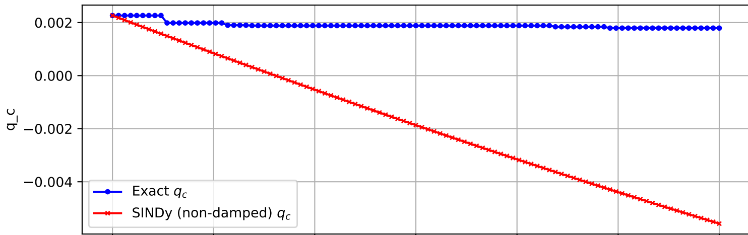
Trajectory 1628 (non-damped)
