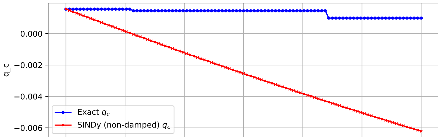
Trajectory 1629 (non-damped)
