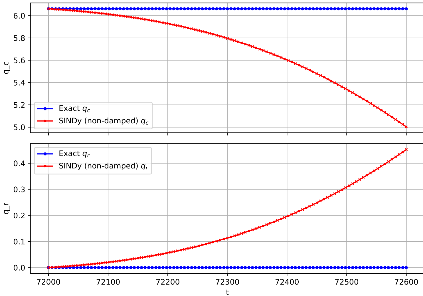
Trajectory 163 (non-damped)
