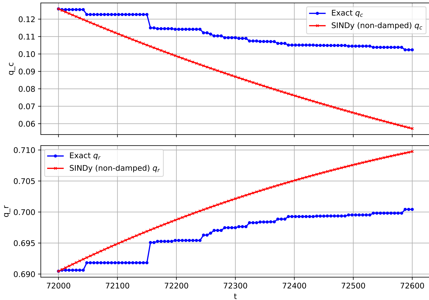
Trajectory 1632 (non-damped)
