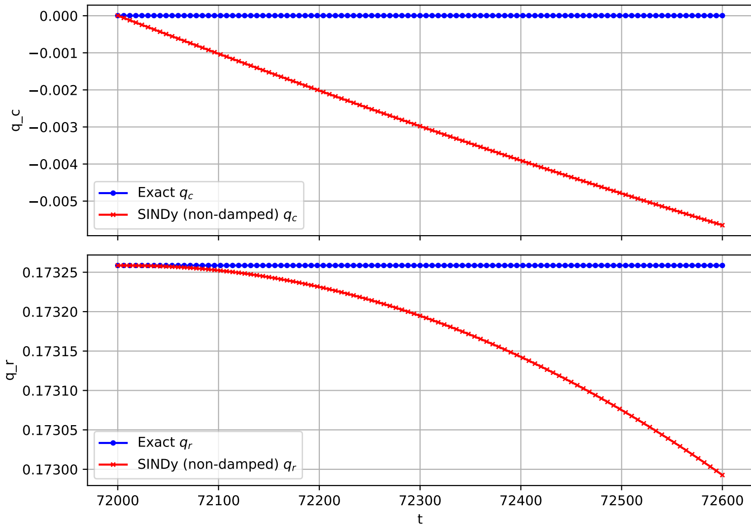
Trajectory 1635 (non-damped)
