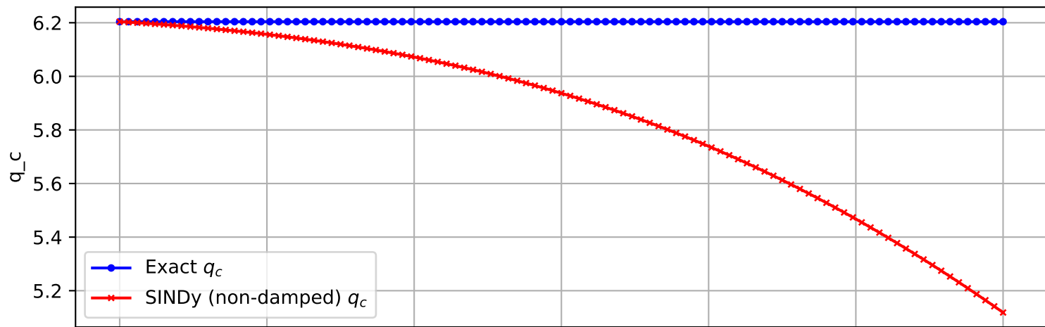
Trajectory 1642 (non-damped)
