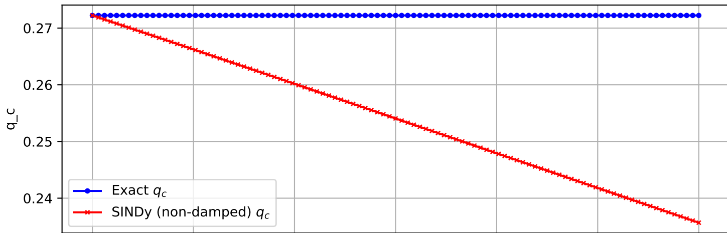
Trajectory 1656 (non-damped)
