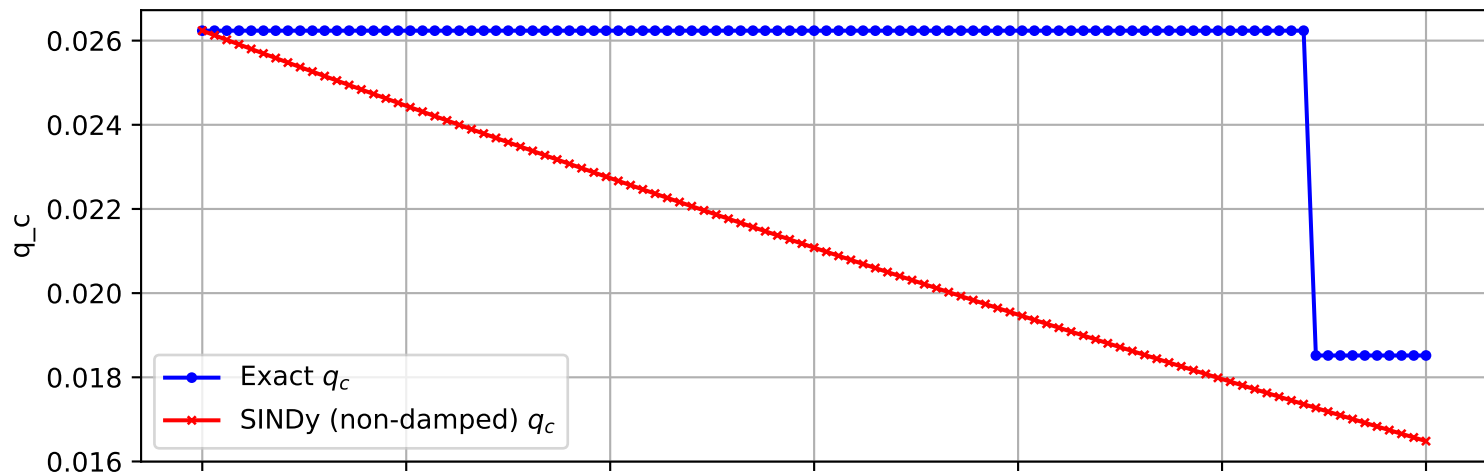
Trajectory 1668 (non-damped)
