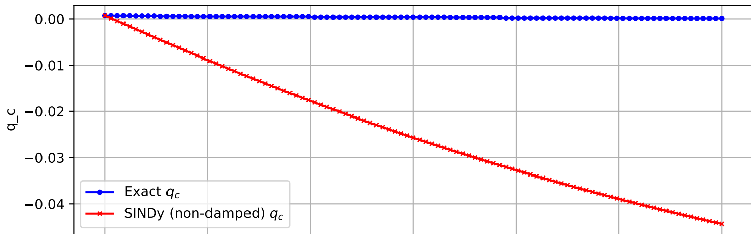
Trajectory 1695 (non-damped)
