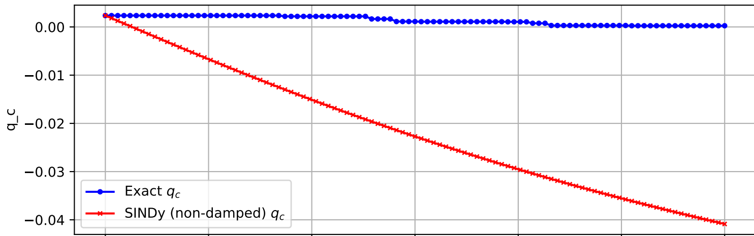
Trajectory 1698 (non-damped)
