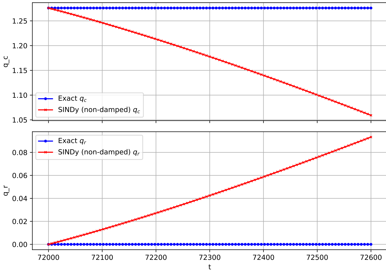
Trajectory 17 (non-damped)
