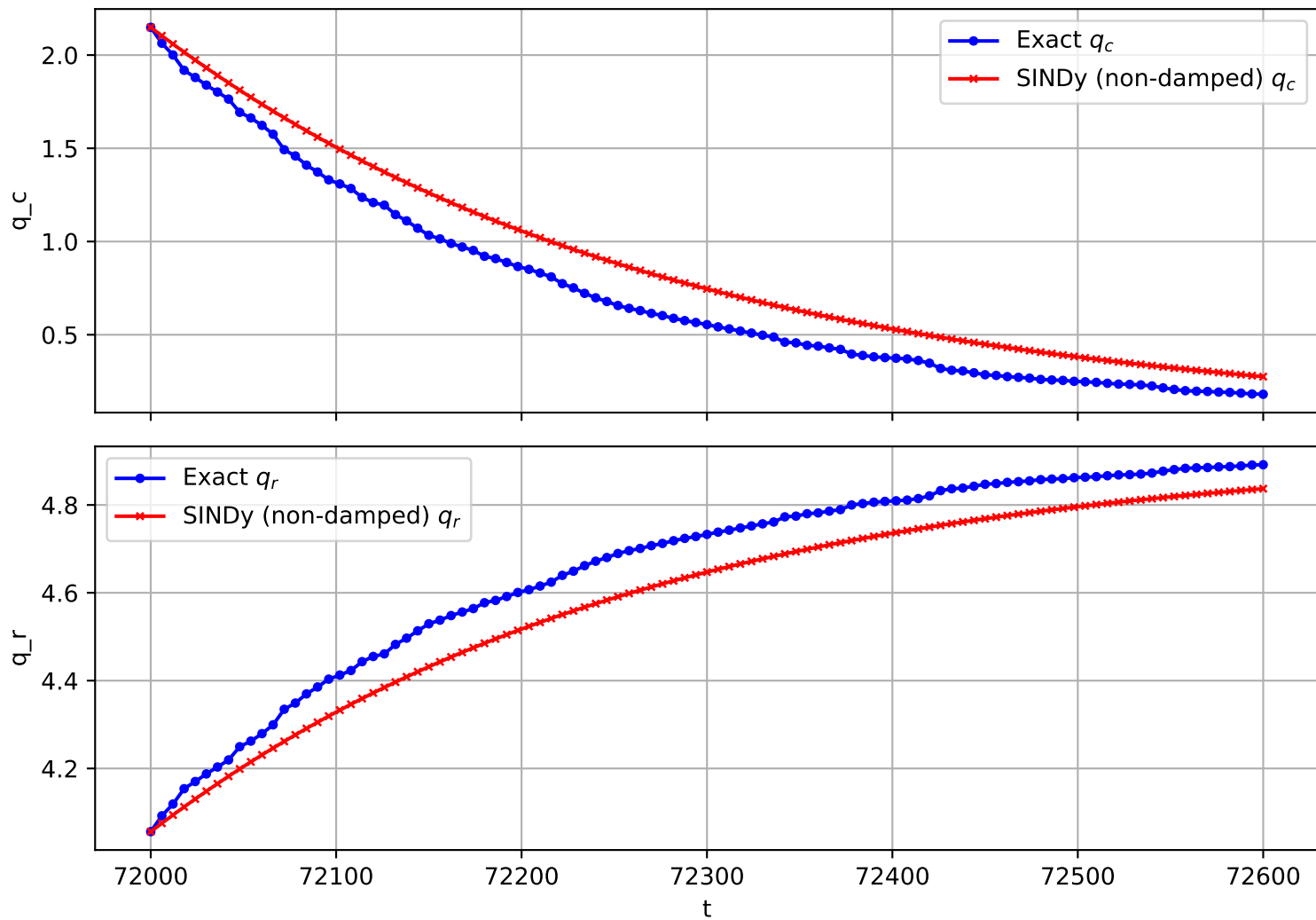
Trajectory 1703 (non-damped)
