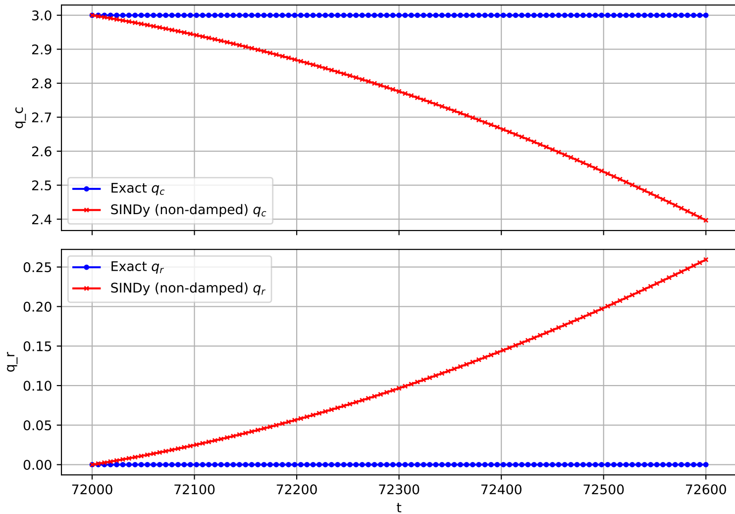
Trajectory 1706 (non-damped)
