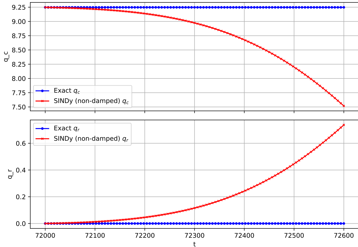
Trajectory 171 (non-damped)
