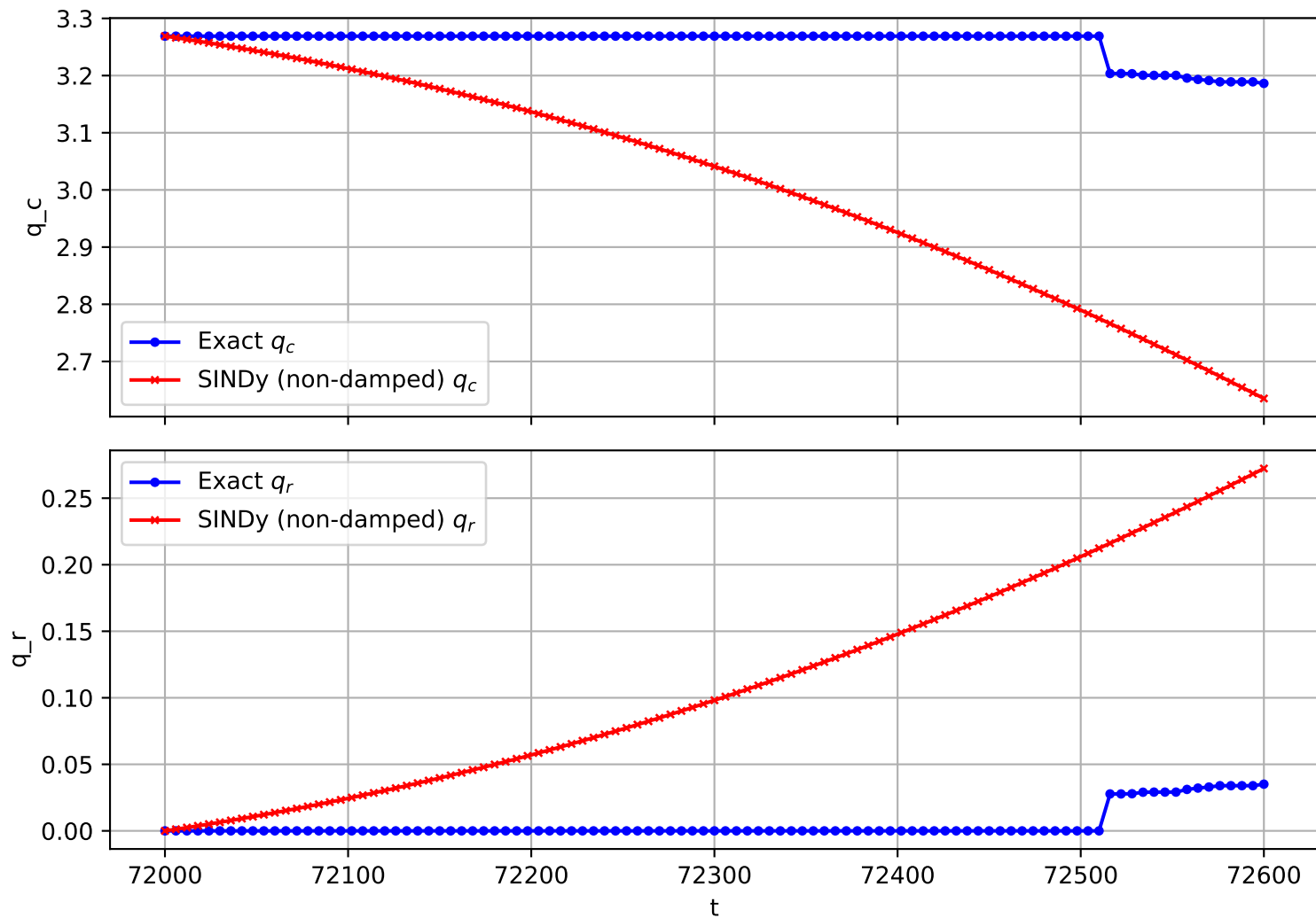
Trajectory 1712 (non-damped)
