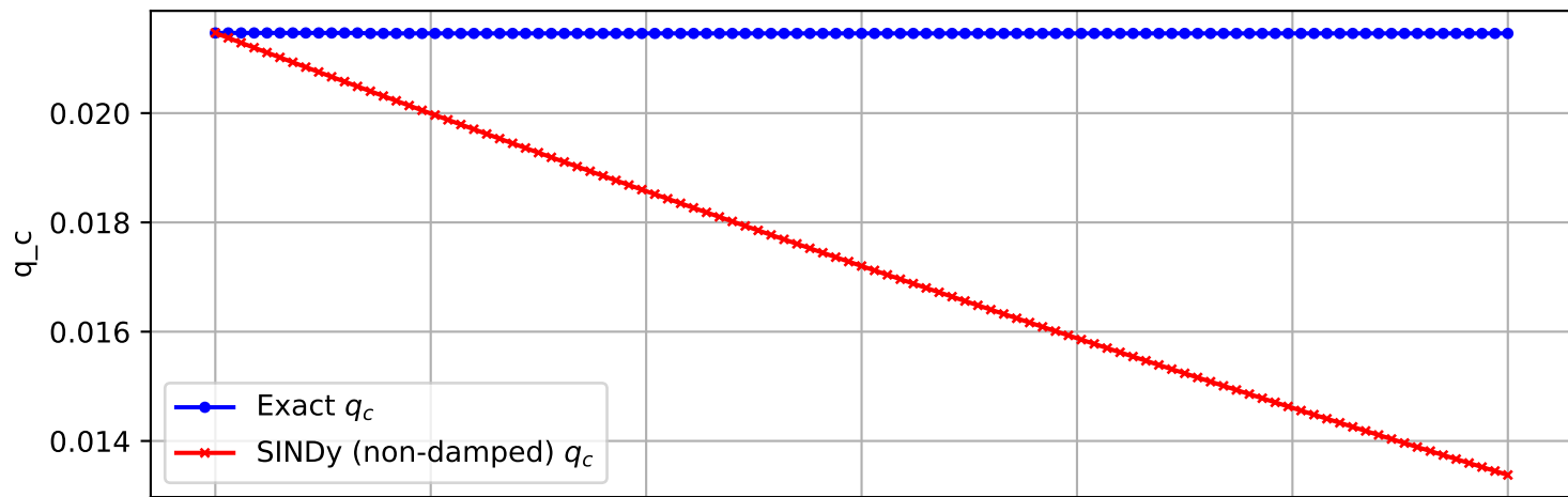
Trajectory 1716 (non-damped)
