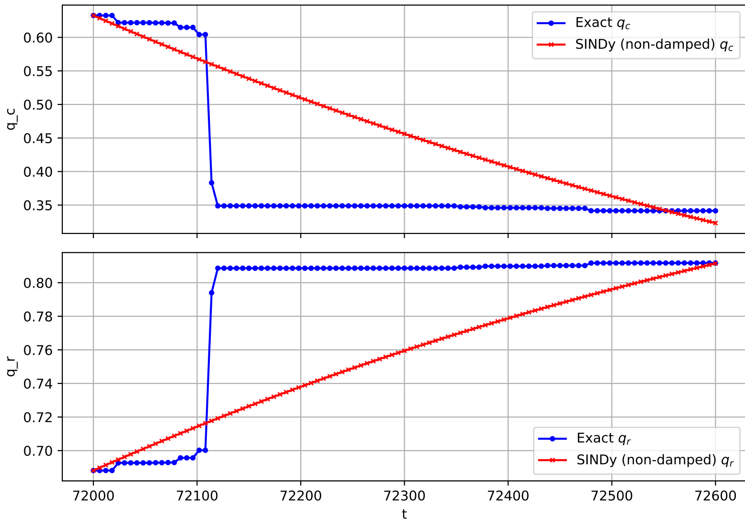
Trajectory 1718 (non-damped)
