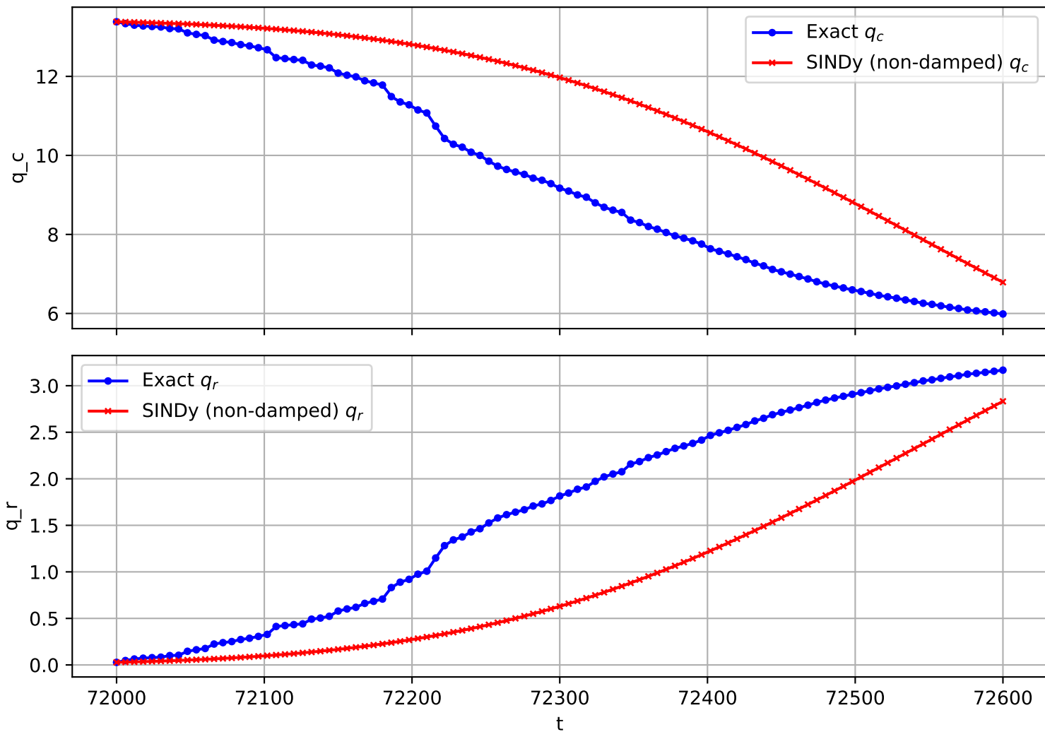
Trajectory 172 (non-damped)
