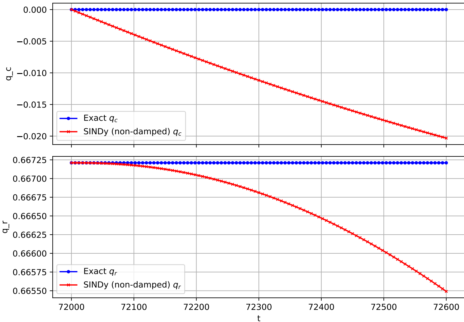
Trajectory 1721 (non-damped)
