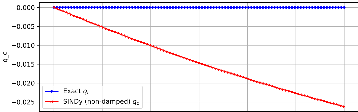
Trajectory 1724 (non-damped)
