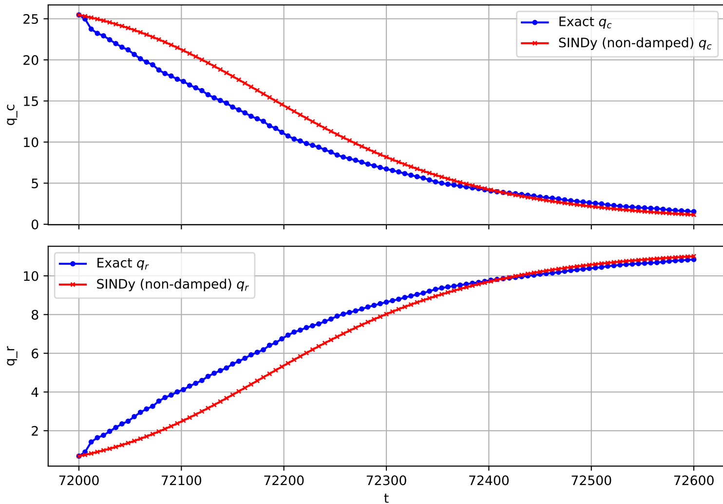
Trajectory 174 (non-damped)
