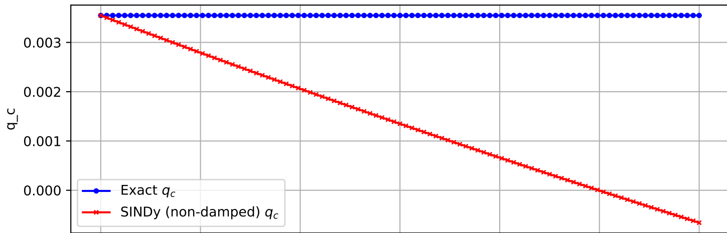
Trajectory 1747 (non-damped)
