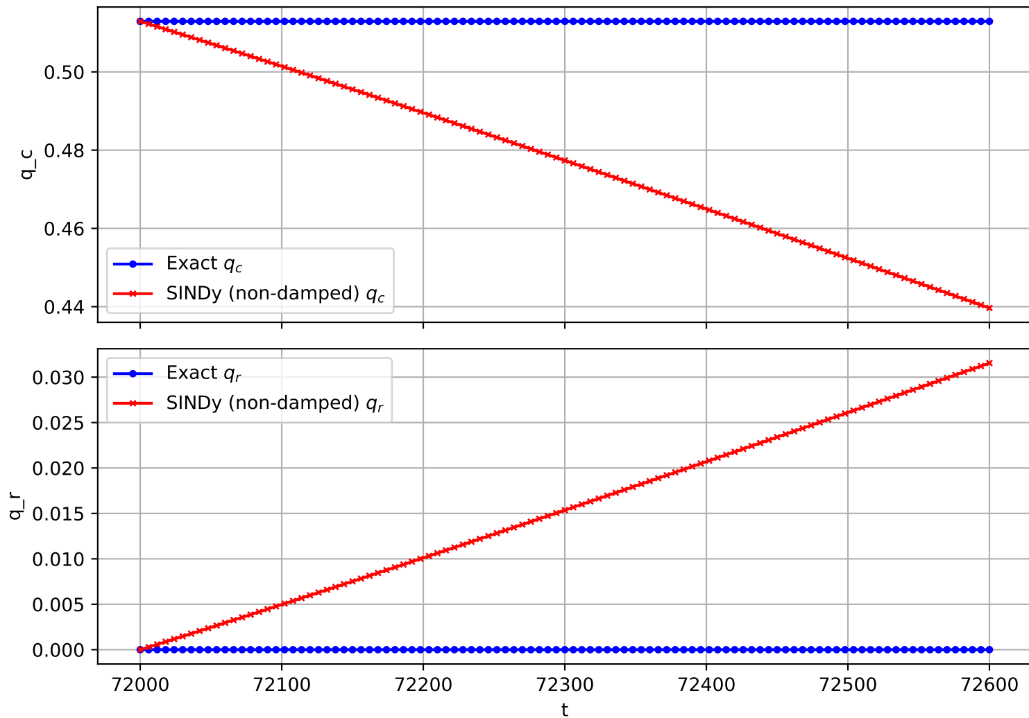
Trajectory 1753 (non-damped)
