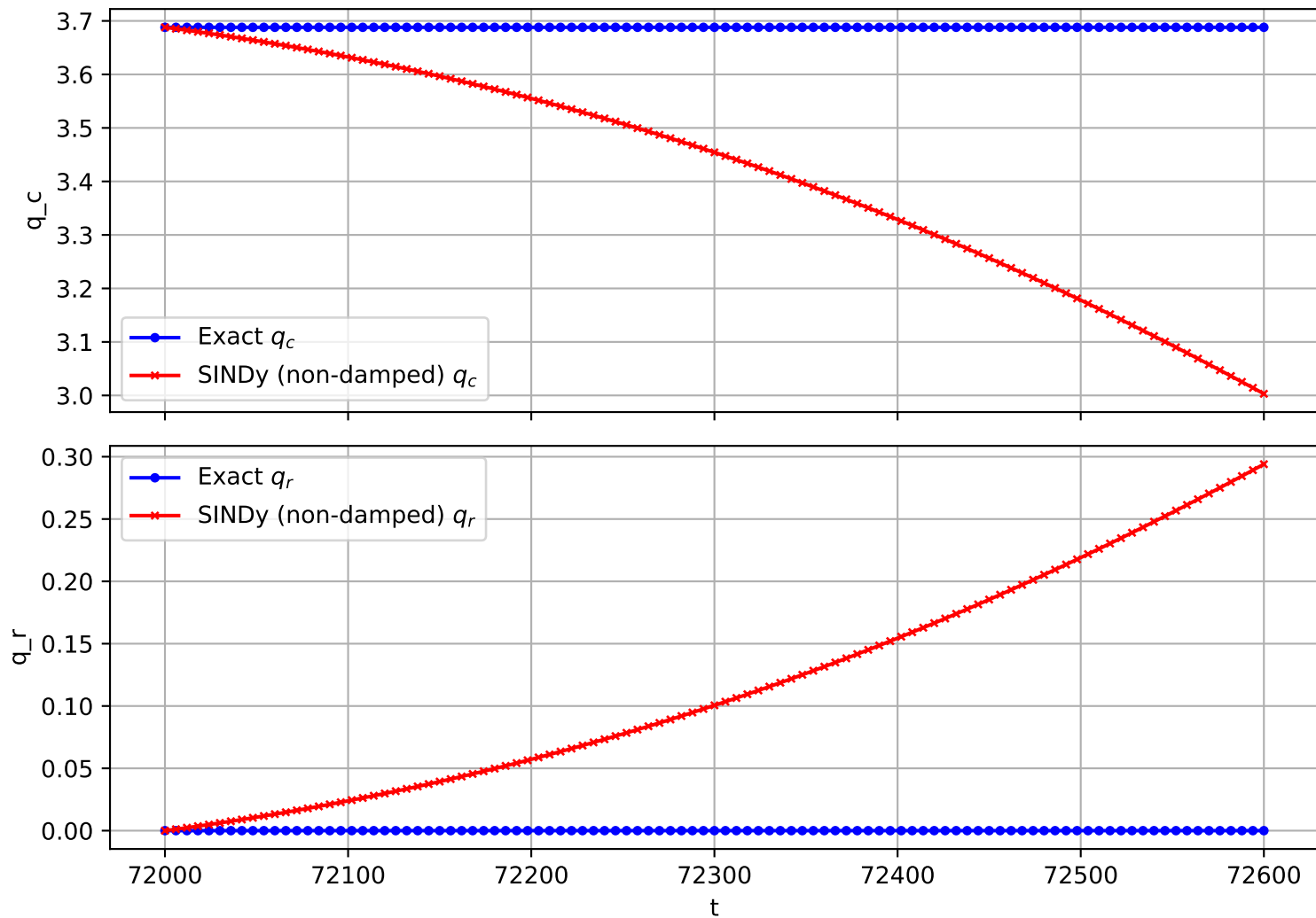
Trajectory 1760 (non-damped)
