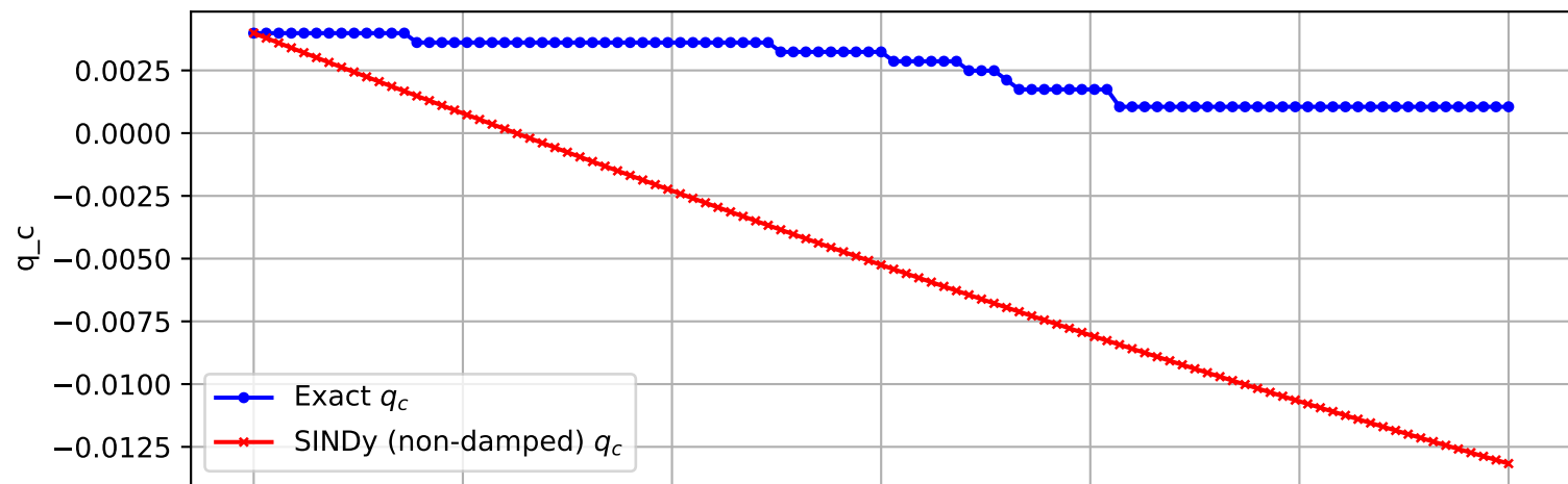
Trajectory 1766 (non-damped)
