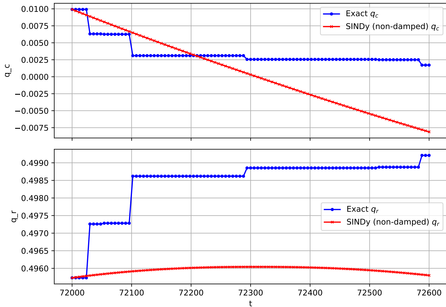
Trajectory 1767 (non-damped)
