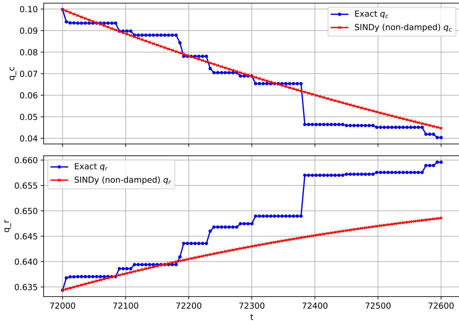
Trajectory 1768 (non-damped)
