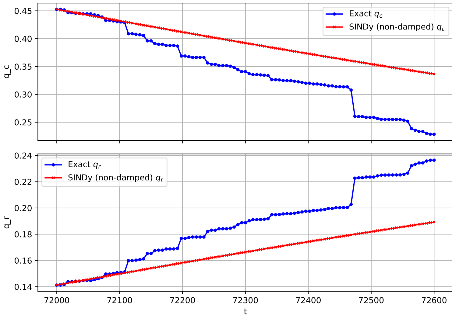
Trajectory 1779 (non-damped)
