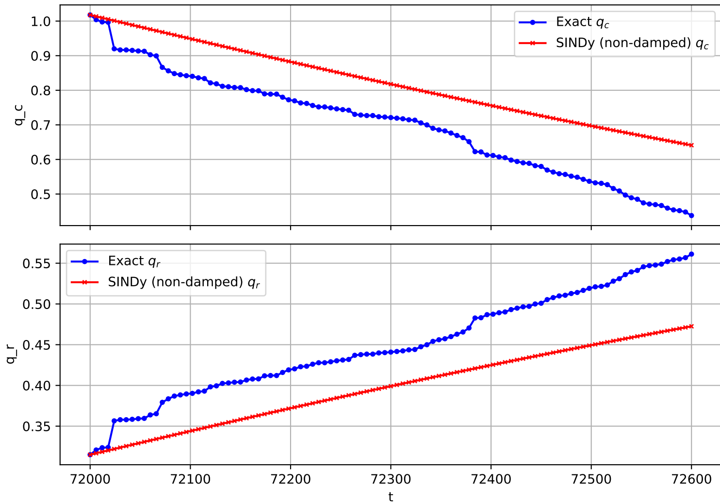
Trajectory 1790 (non-damped)
