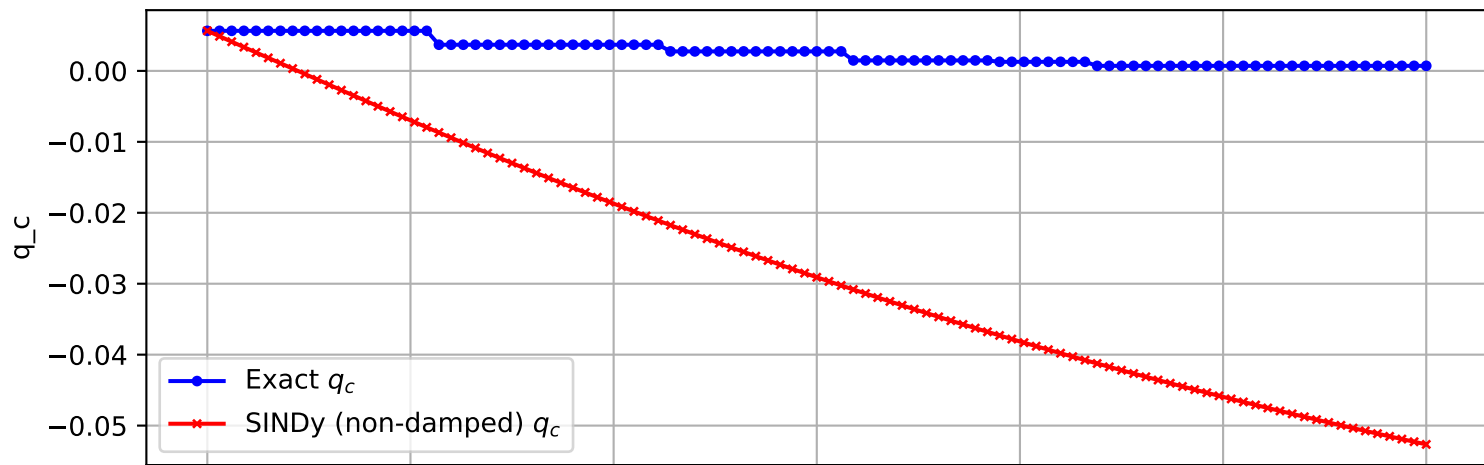
Trajectory 1795 (non-damped)
