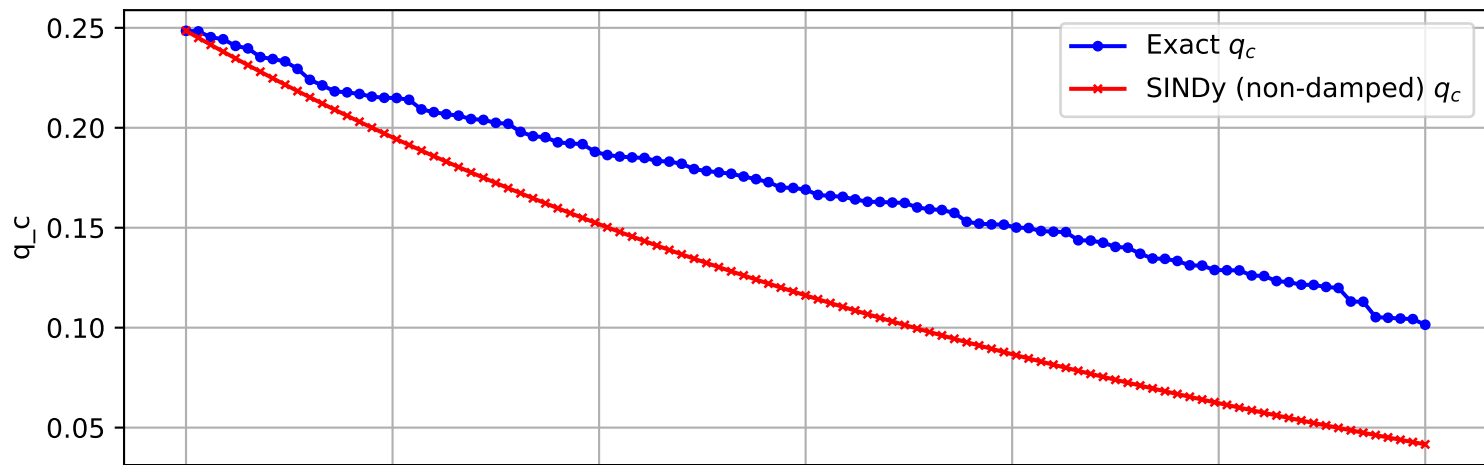
Trajectory 1798 (non-damped)
