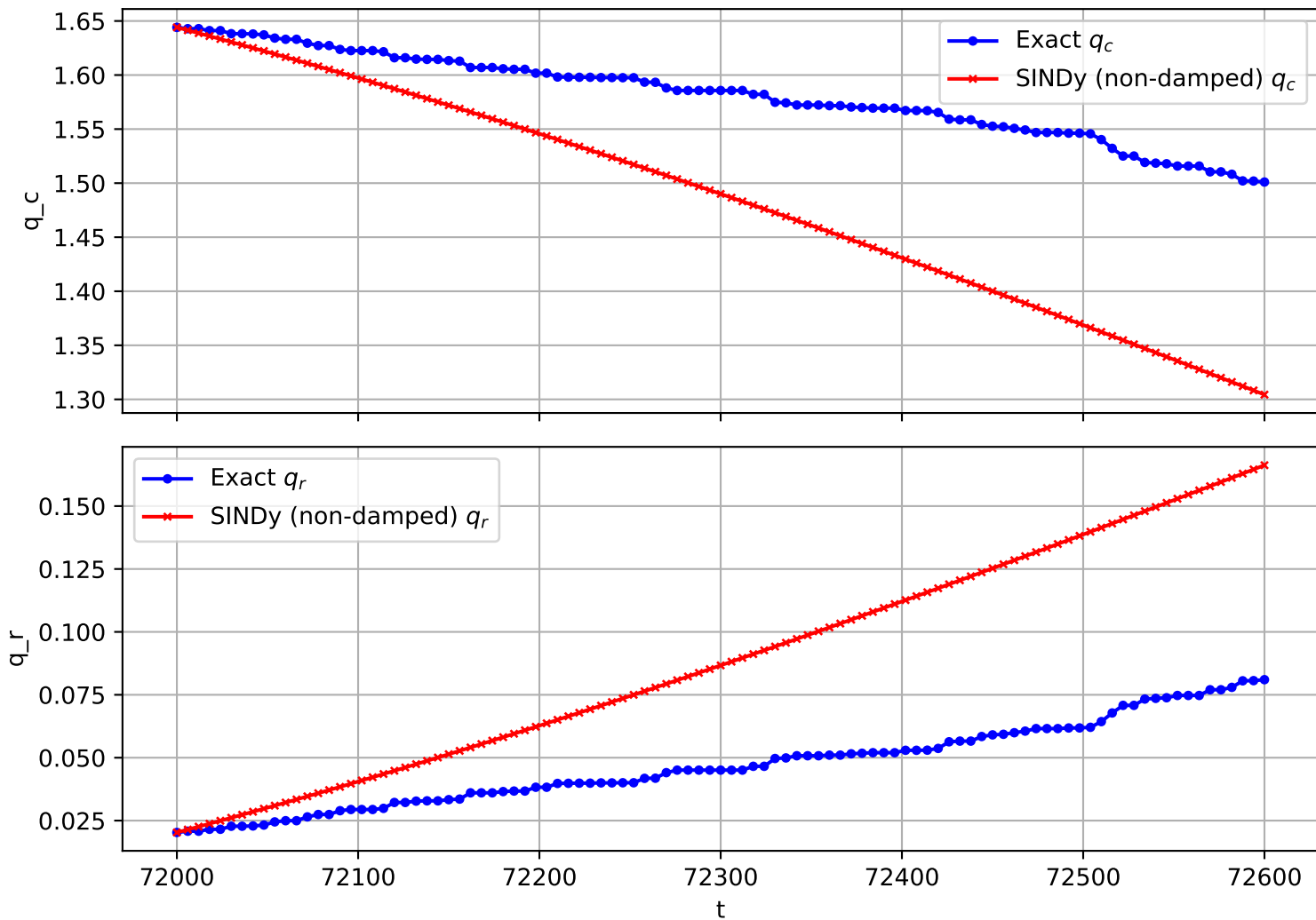
Trajectory 1806 (non-damped)
