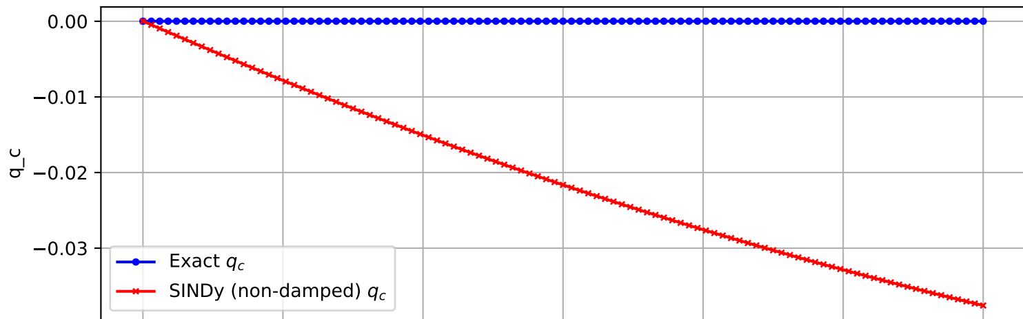
Trajectory 1807 (non-damped)
