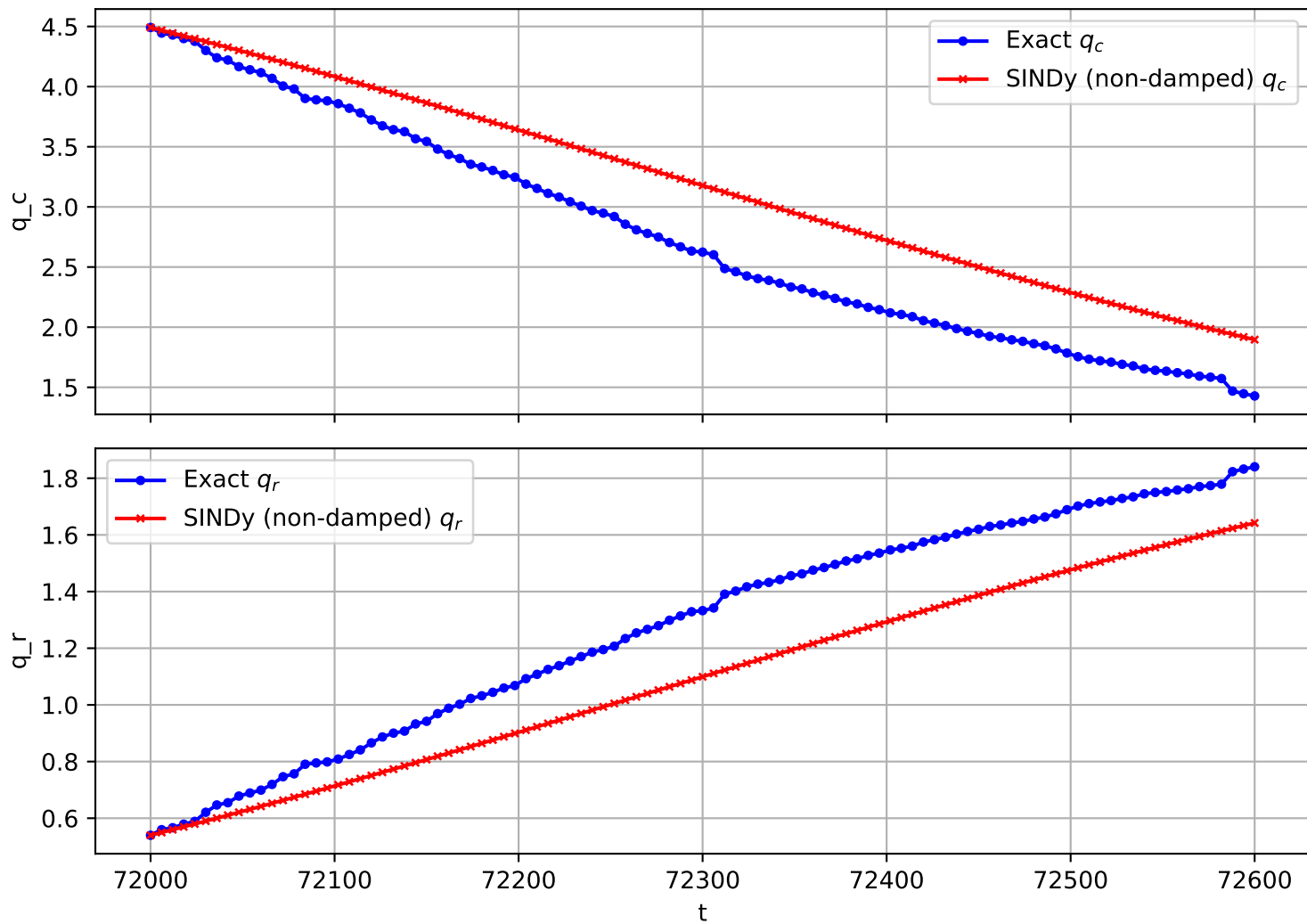
Trajectory 1812 (non-damped)
