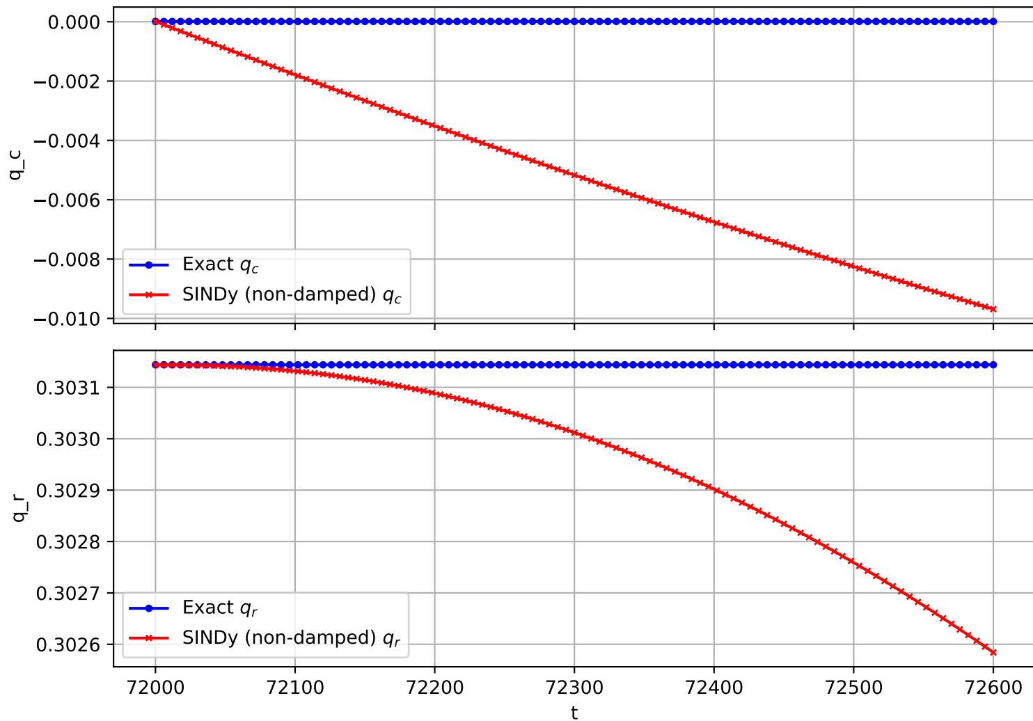
Trajectory 1814 (non-damped)
