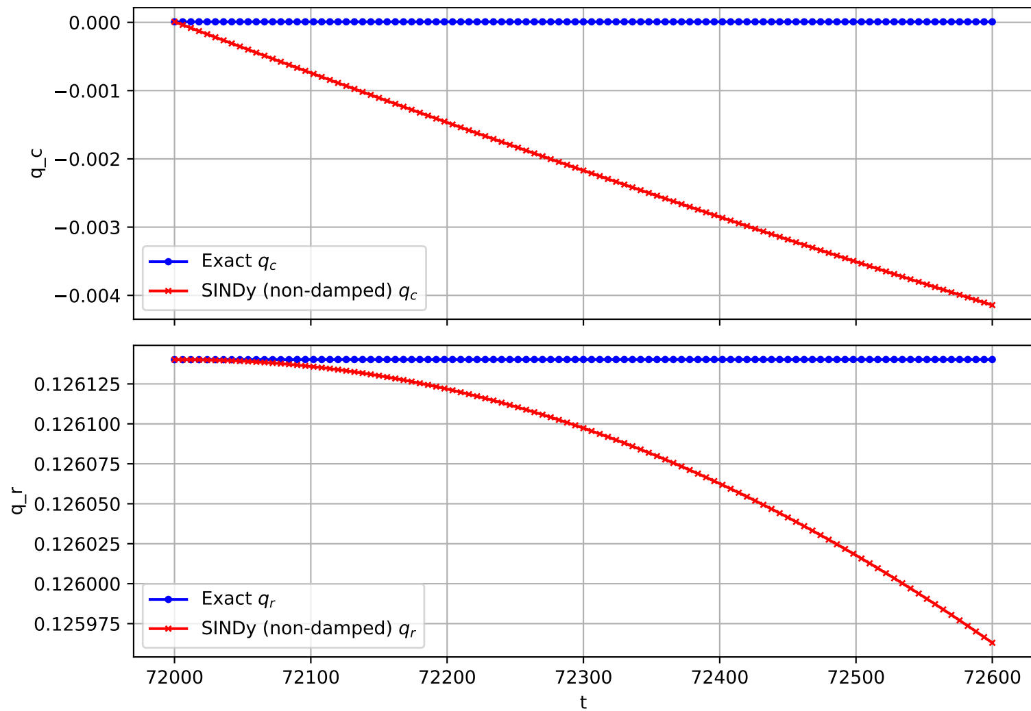
Trajectory 1815 (non-damped)
