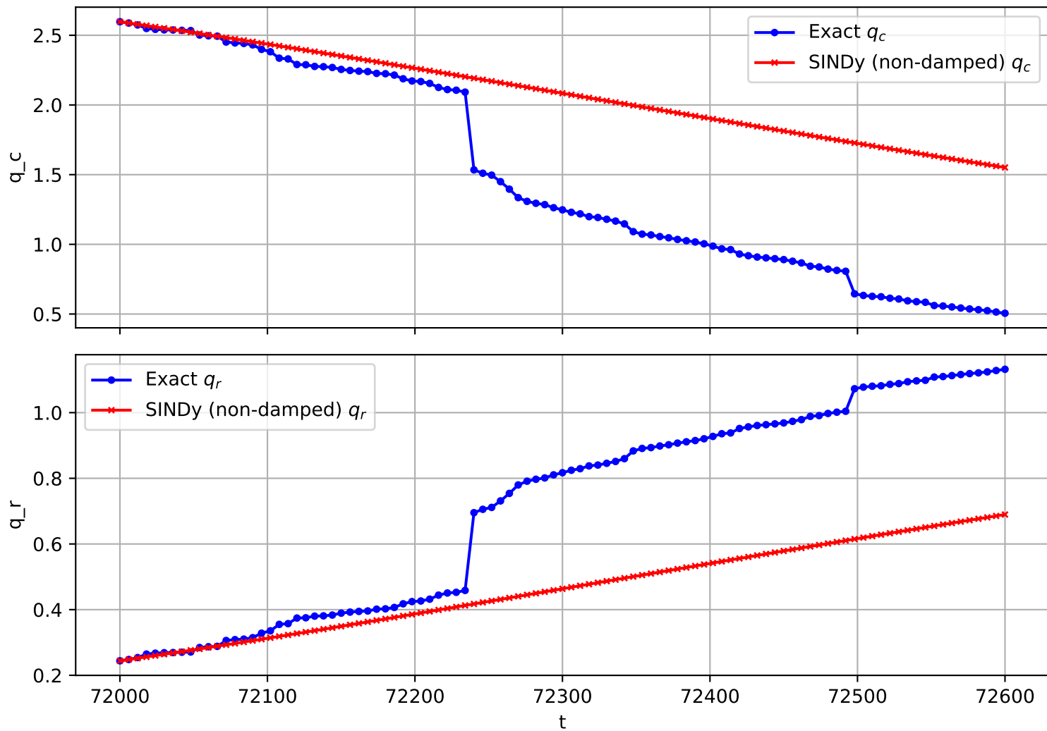
Trajectory 1819 (non-damped)
