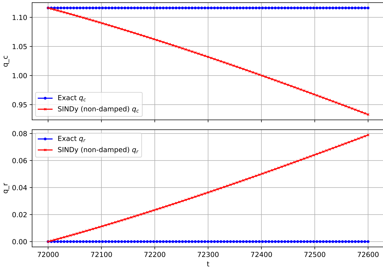
Trajectory 1836 (non-damped)
