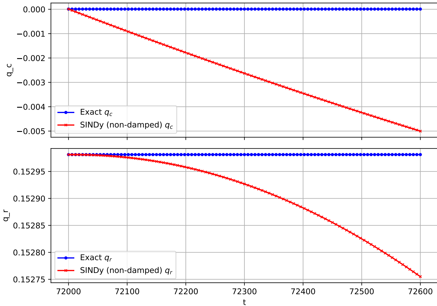
Trajectory 1846 (non-damped)
