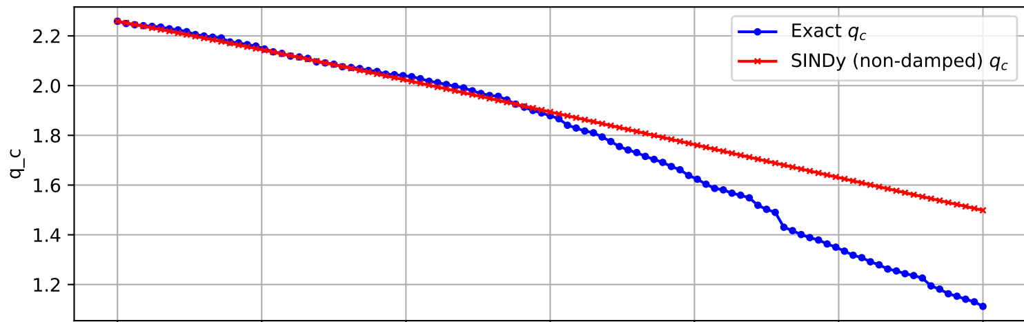
Trajectory 1853 (non-damped)
