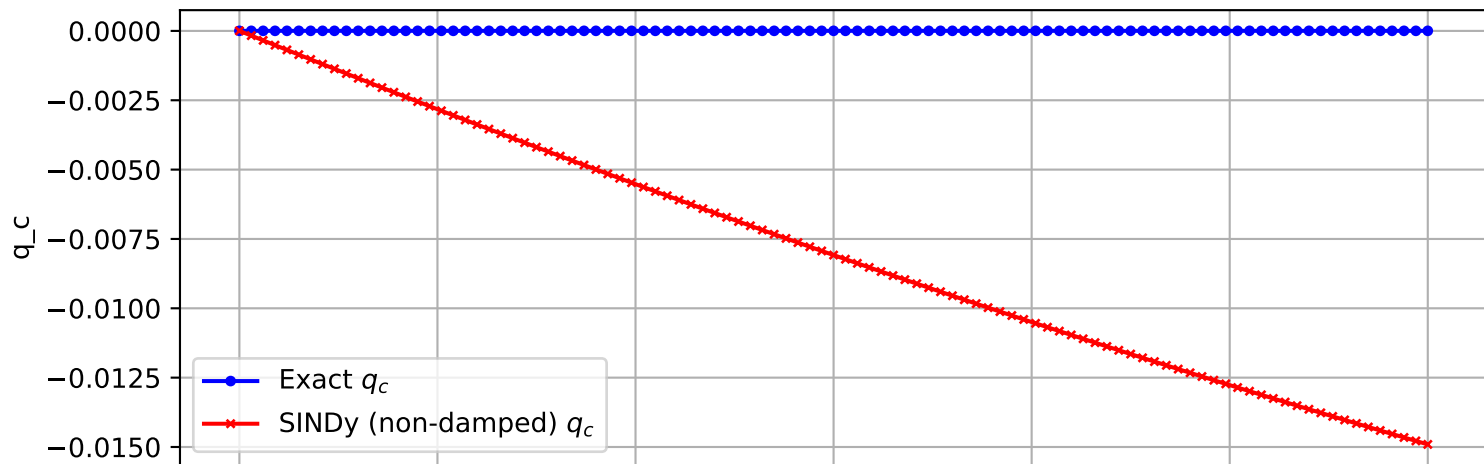
Trajectory 1858 (non-damped)
