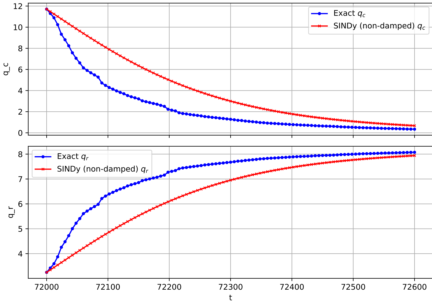
Trajectory 186 (non-damped)
