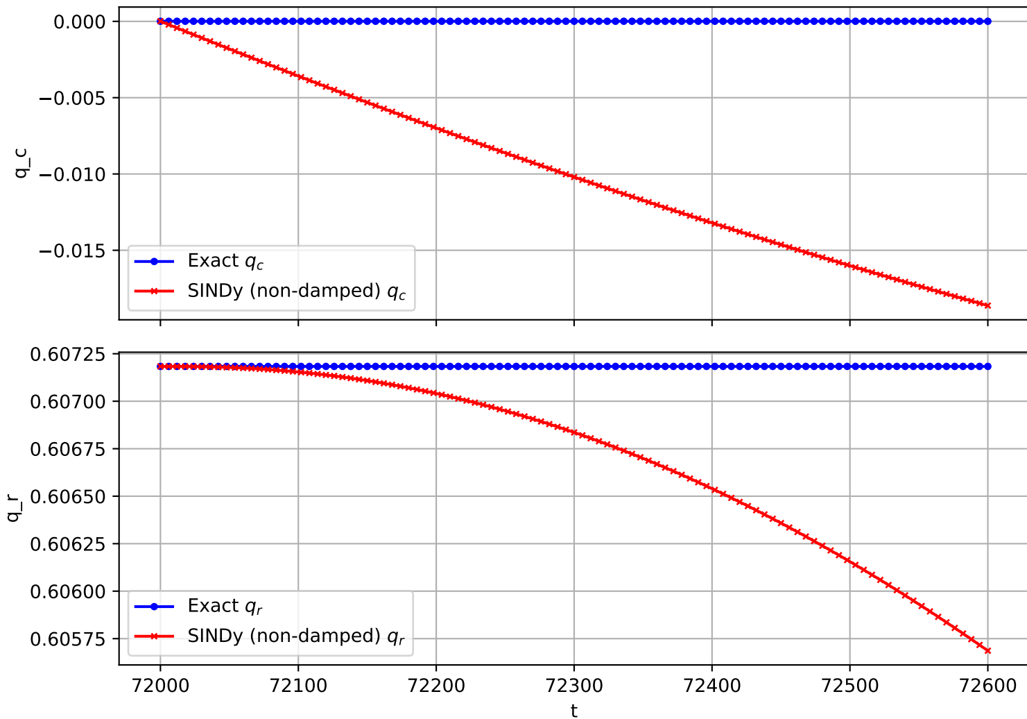
Trajectory 1860 (non-damped)
