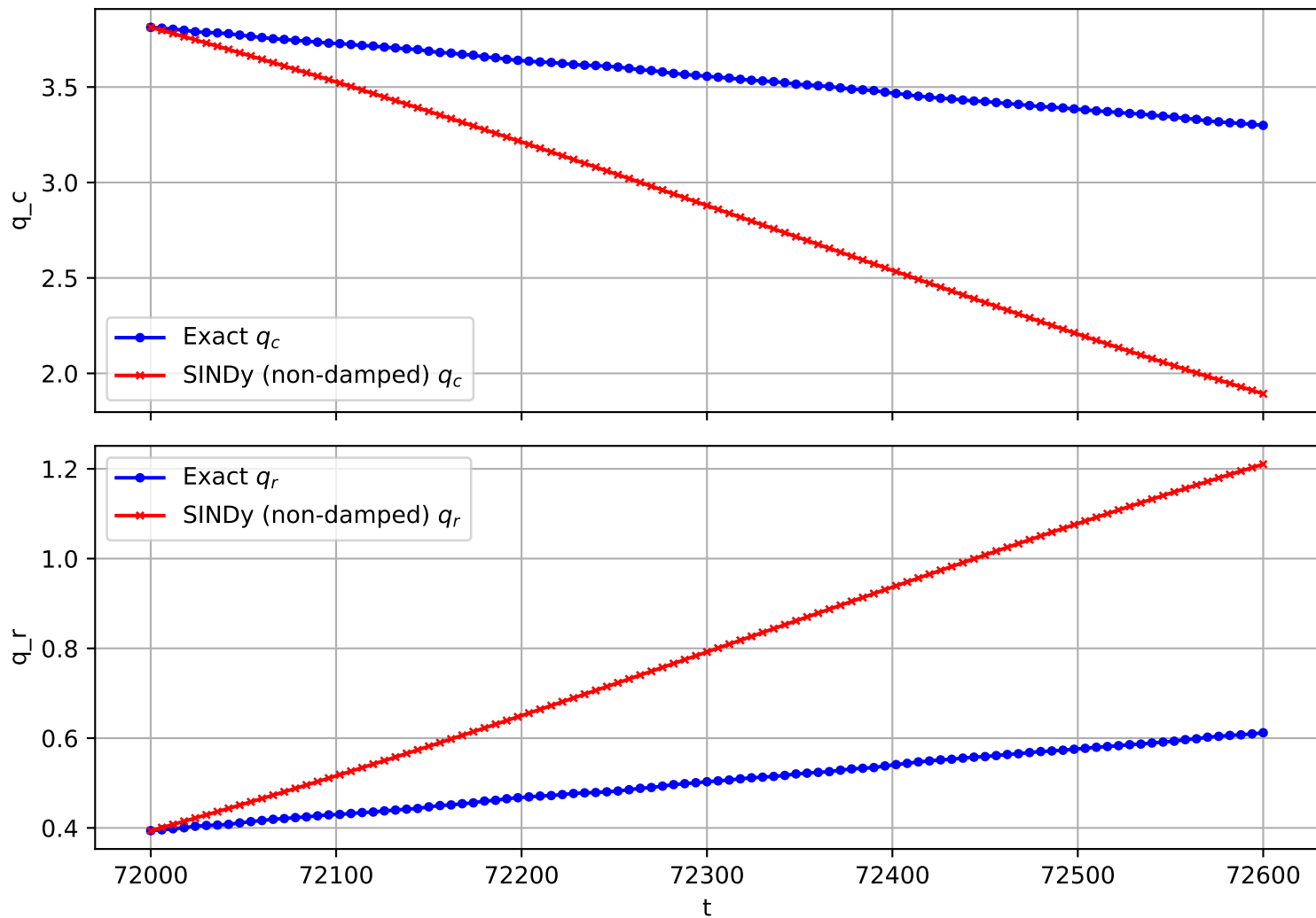
Trajectory 1864 (non-damped)
