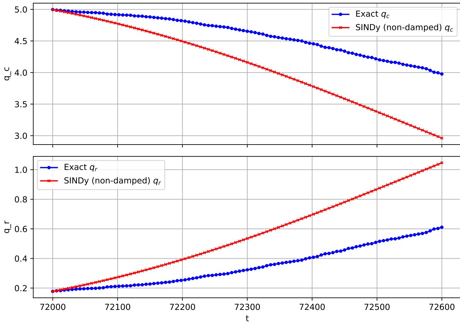
Trajectory 1865 (non-damped)
