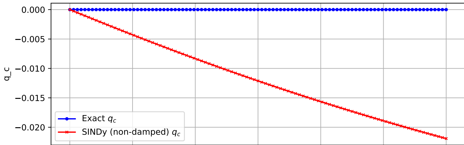
Trajectory 1874 (non-damped)
