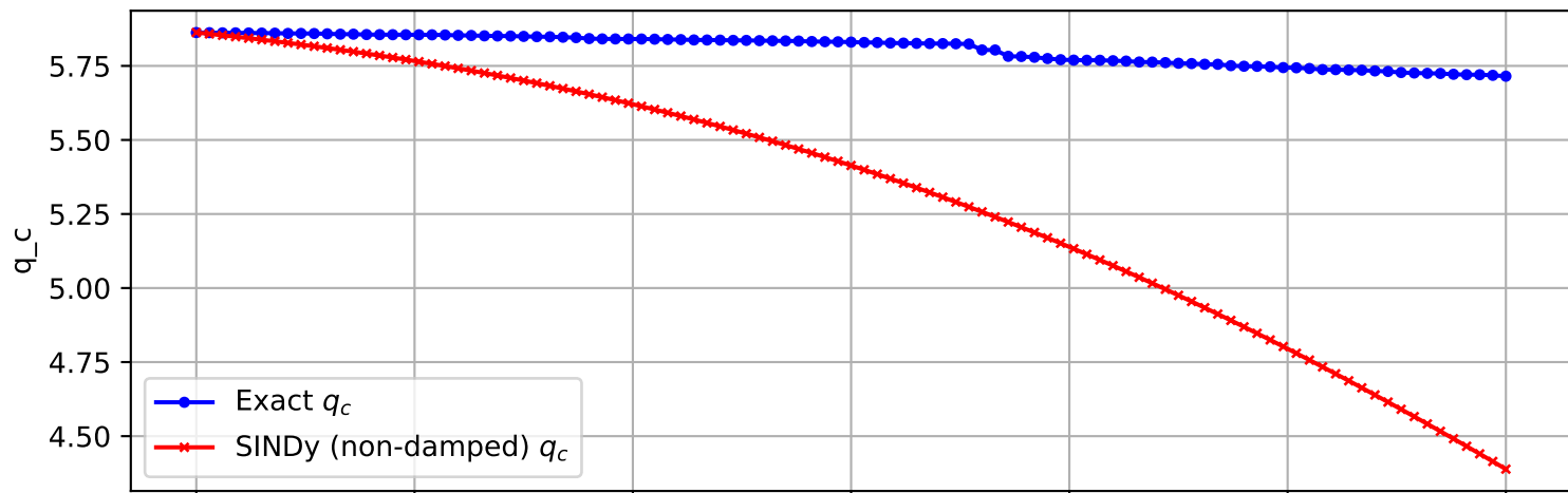
Trajectory 1882 (non-damped)
