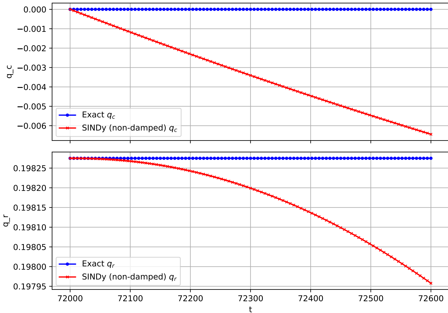
Trajectory 1888 (non-damped)
